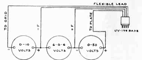
Fig. 9. Circuit Tester Diagram.
