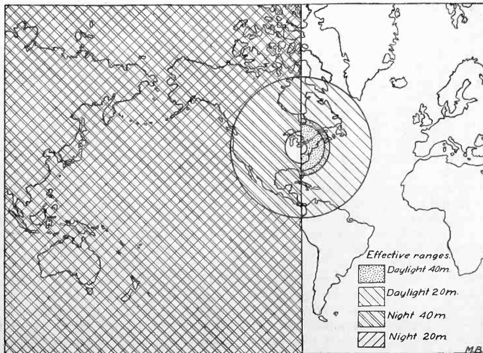
Fig. 5. Approximate Ranges to Be Expected from Efficient 40 and 20 Meter Installations. An 80 Meter Wave Is Necessary to Close the Gap Adjacent to the Station.
