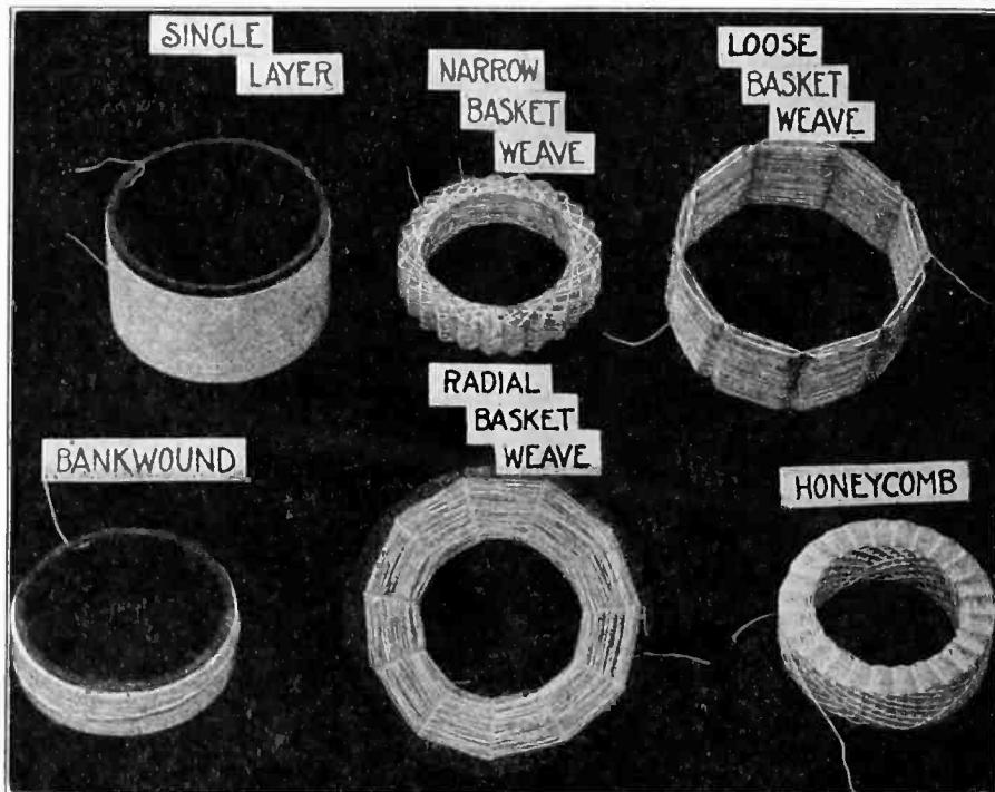
Low-Loss Coils Used for Measurements
