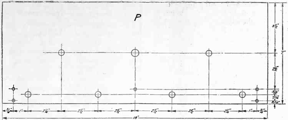
Fig. 2. Layout for Main Panel.
