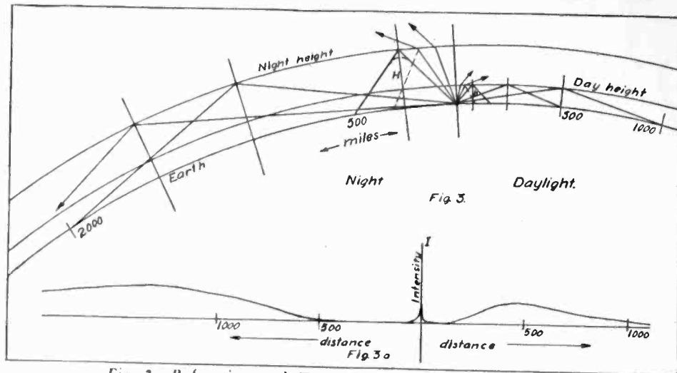
Fig. 3. Refraction and Total Reflection of 40 Meter Signals. Fig. 3a. Resultant Audibility Curve.
