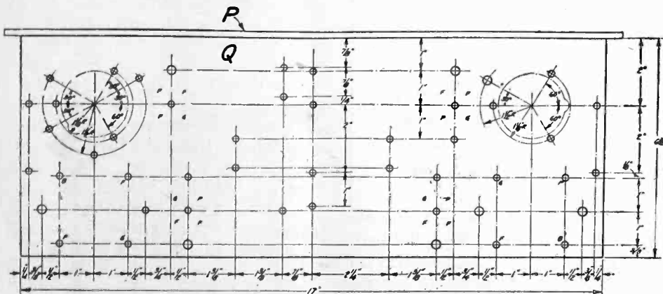
Fig. 3. Sub-panel Layout.
