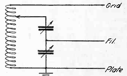
FIG. 2 Colpitts System
