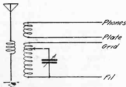
FIG. 3 Standard "3" Circuit
