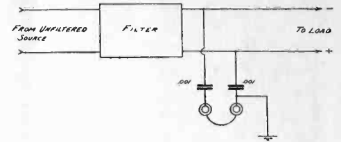
Fig. 4. Test Circuit for Determining Effectiveness of Filter.
