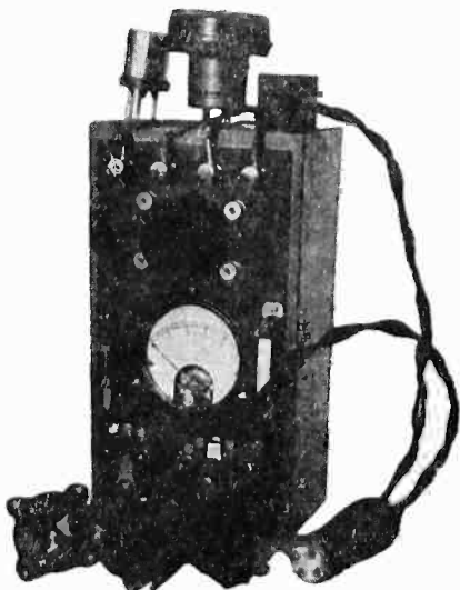
Fig. 4. Tube Tester.
