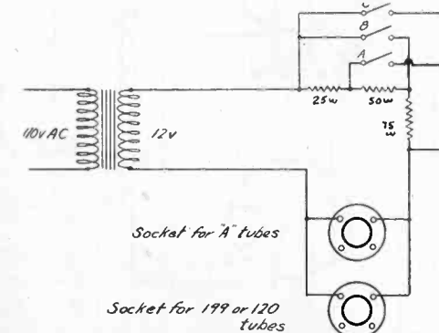
Fig. 2. Connections for Home-Made Tube Rejuvenator.
