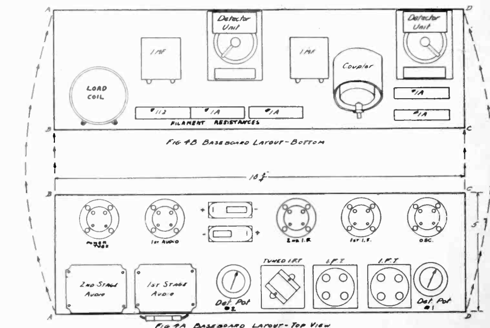
Fig. 4. (a) Top View of Shelf, Showing Actual Position of Apparatus; (b) Under Part of Shelf.
