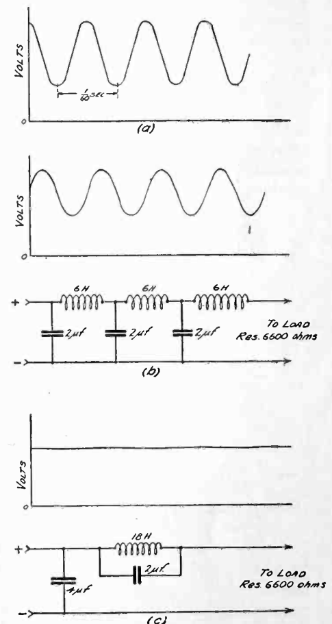
Fig. 5. Example of Improperly Designed Filters.
