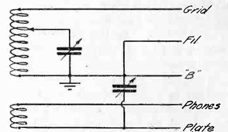
FIG. 4 Capacity Controlled Feedback
