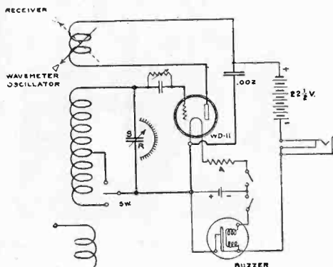
Fig. 3. Circuit Diagram of Wavemeter Oscillator.
