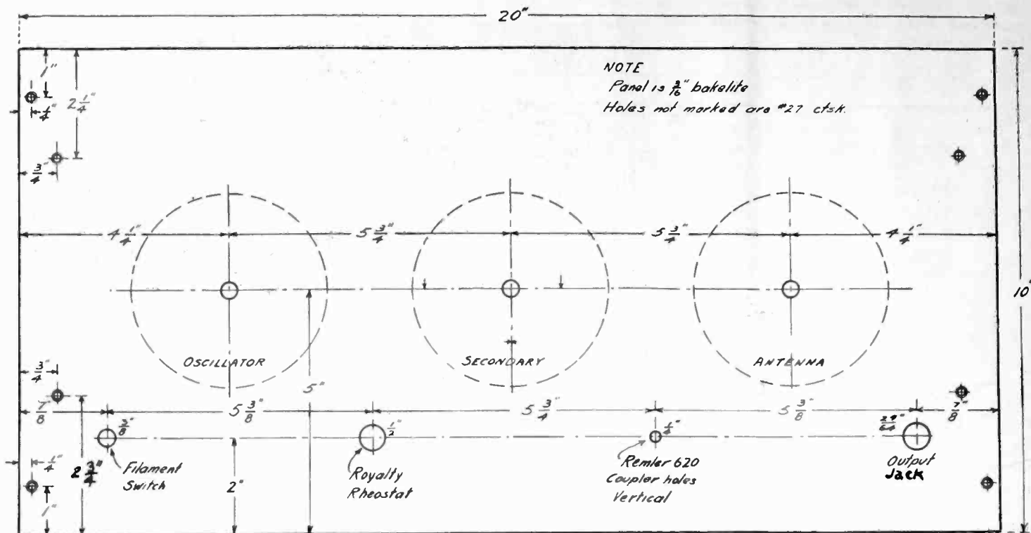
Fig. 3. Template for Drilling Panel.
