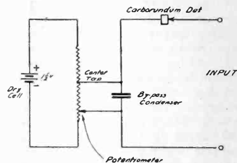
Fig. 1. Circuit of Carborundum Detector Unit.
