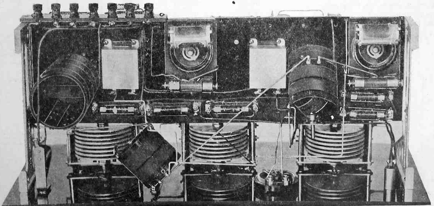
Bottom View of Shelf, With Wiring Details.
