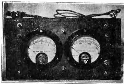
Fig. 6. Voltmeter-Milliammeter Combination.
