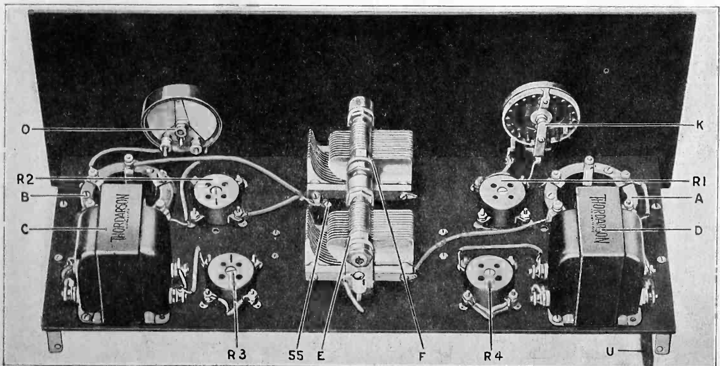
Rear View Showing Top of Sub-Panel.
